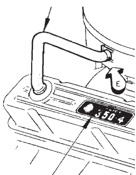
Breather Tube
